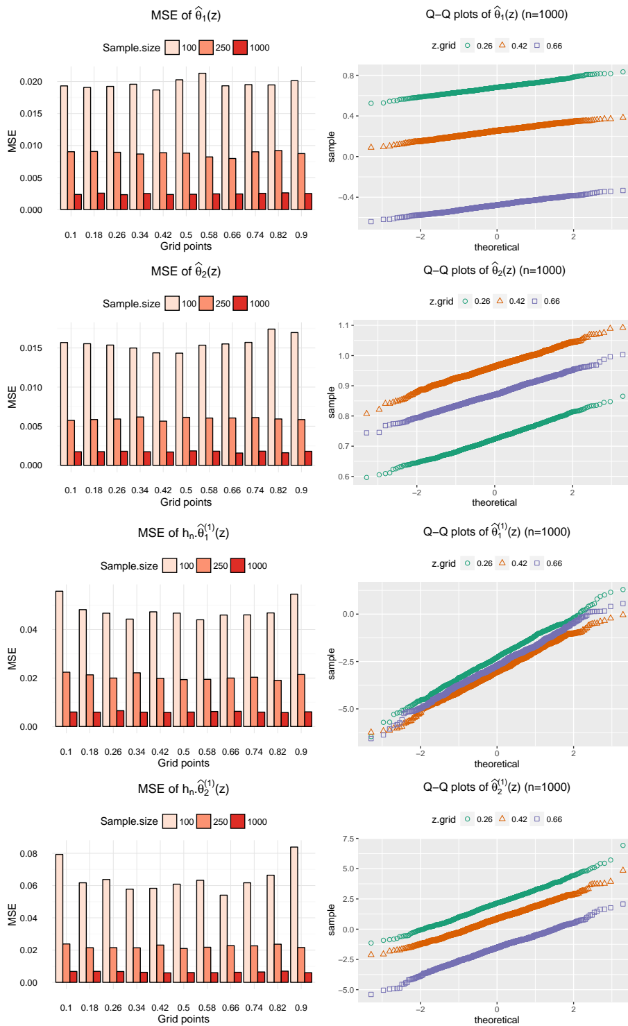
Fig. 1 Results from the simulation study based on 1000 simulated data sets. The first column displays the mean squared errors of \hat{\theta}_1 , \hat{\theta}_2 , h_n \hat{\theta}_1^{(1)} and h_n \hat{\theta}_2^{(1)} for different sample sizes. The second column displays QQ-plots for n = 1000 of estimates of \hat{\theta}_1 , \hat{\theta}_2 , \hat{\theta}_1^{(1)} and \hat{\theta}_2^{(1)} .
